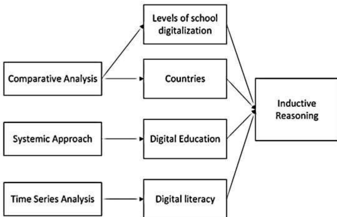
Figure 1. Methodology
